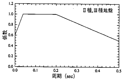
Fig. 4 上下動変換係数スペクトル Maximum Response Acceleration Spectrum to Vertical Ground Motion
